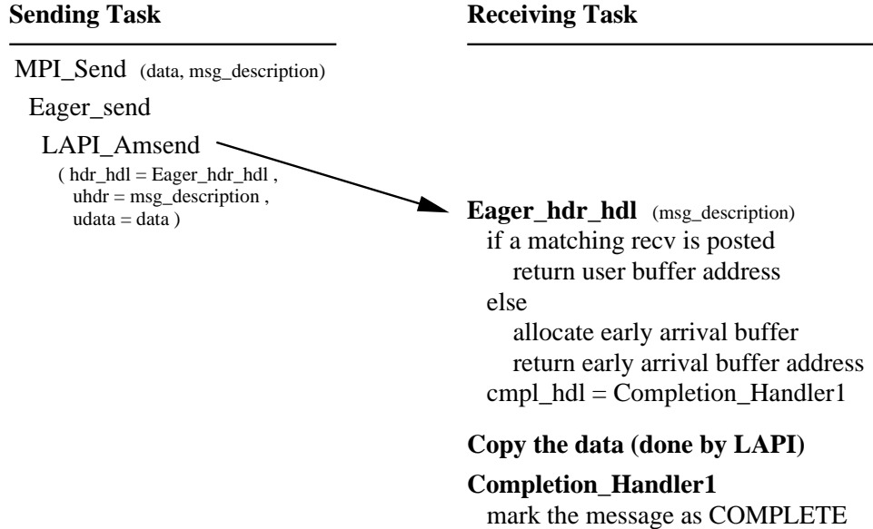
Figure 10: Outline of MPI_Send and the sequence of actions taken at the sending and receiving tasks when the message size is less than the Eager Limit.
