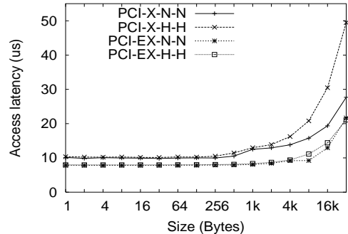
Figure 2. Host/NIC Memory Access Latency
