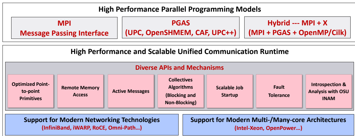
Figure 1: MVAPICH2-X Architecture
